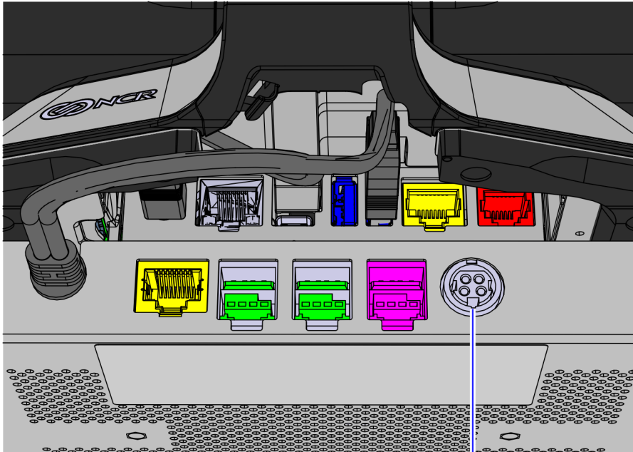
Power In
