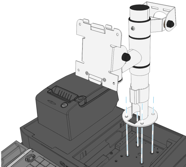
INTEGRATION TRAY
